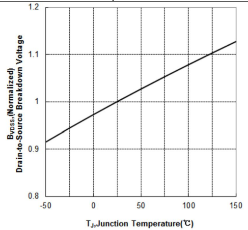
Typical Breakdown Voltage vs Junction Temperature
