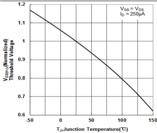
Typical Theshold Voltage vs Junction Temperature
