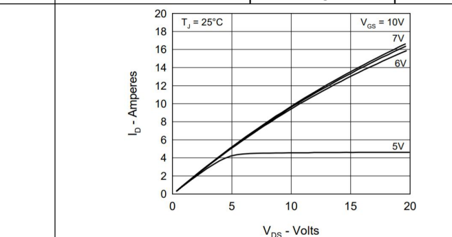
Typical Output Characteristics
