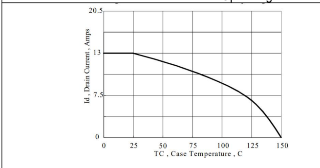
Maximum Continuous Drain Current vs Case Temperature
