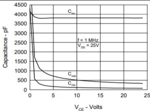
Typical Capacitance vs Drain to Source Voltage
