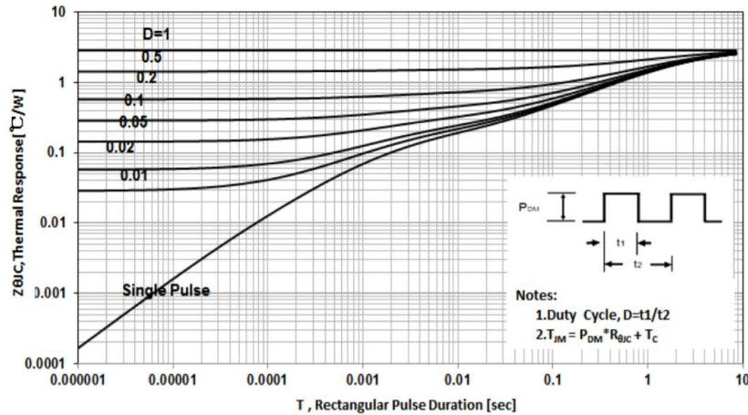
Maximum Effective Thermal Impedance, Junction to Case
