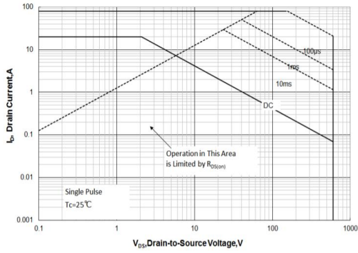
Maximum Forward Bias Safe Operating Area
