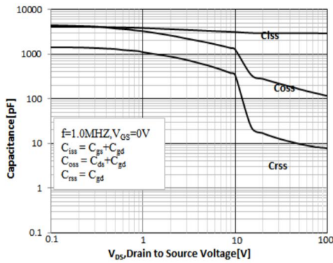
Typical Capacitance vs Drain to Source Voltage
