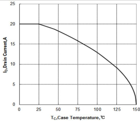
Maximum Continuous Drain Current vs Case Temperature
