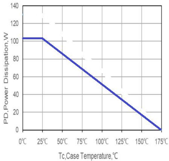
Figure 5. Power De-rating
