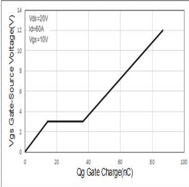
Fig 4. Gate Charge
