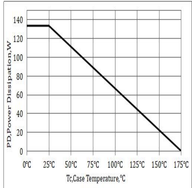
Figure 9. Power De-rating
