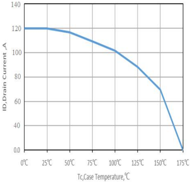
Figure 8. ID Current De-rating
