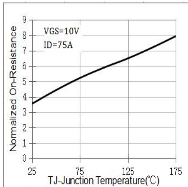
Fig3. Rdson-Junction Temperature
