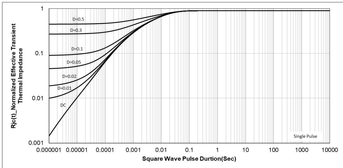
Figure 10 Normalized Maximum Transient Thermal Impedance
