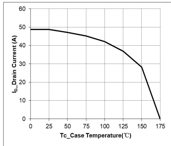
Figure 4 Current De-rating
