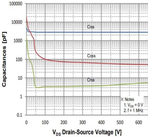
Figure 5. Capacitance Characteristics
