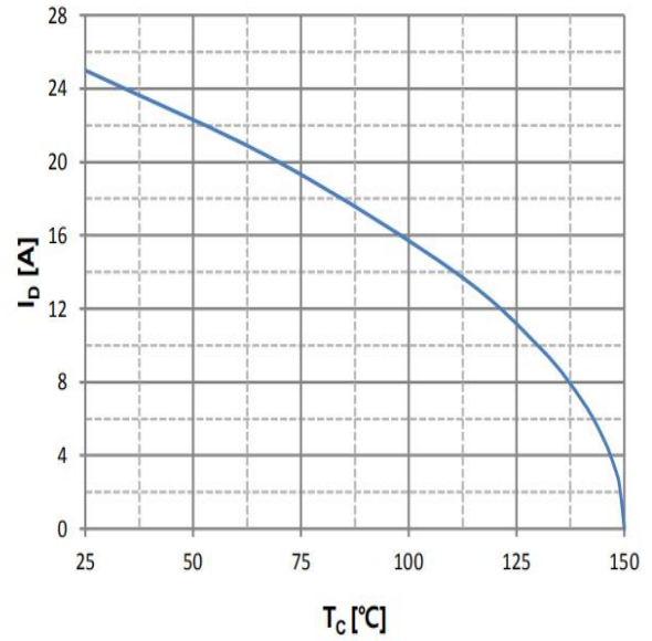
Figure 10. Maximum Drain Current vs. Case Temperature
