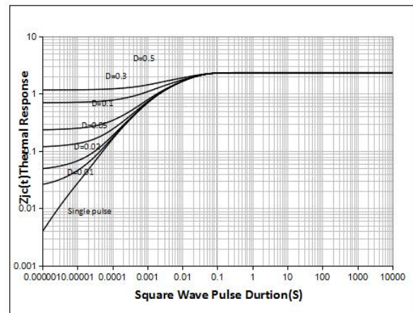
Figure 10. Maximum Transient Thermal Impedance
