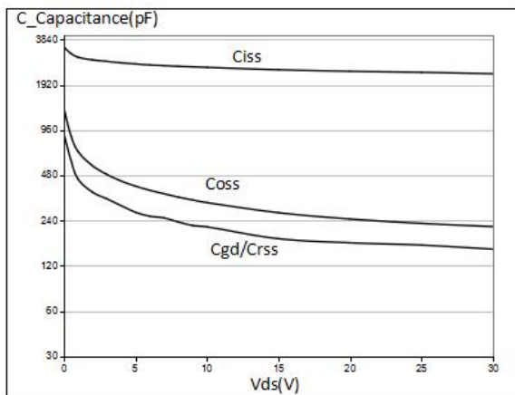
Figure 9. Capacitance vs Vds
