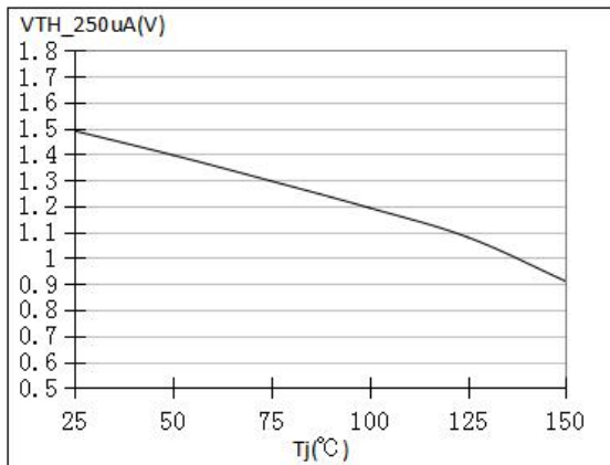
Figure 7. VTH vs. Junction Temperature
