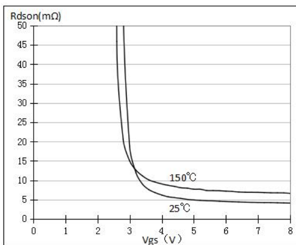
Figure 5. On-resistance vs.Vgs
