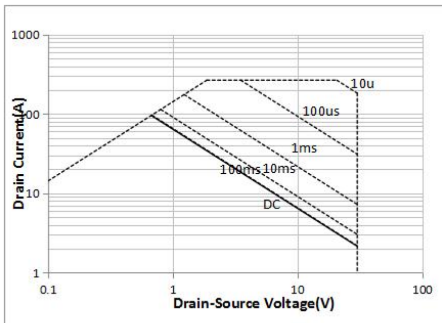
11. Maximum Safe Operating Area
