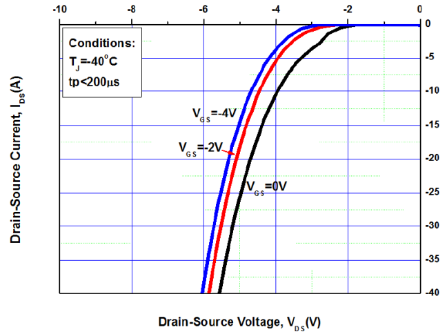
Figure 8. Body Diode Characteristic at -40°C
