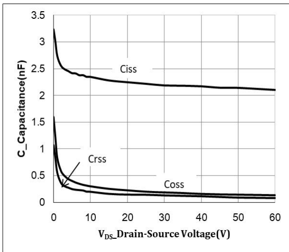
Fig 7 Capacitances vs Vds
