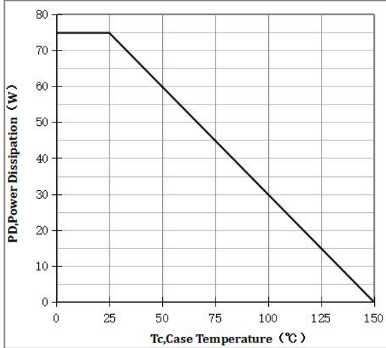
Fig 5 Power De-rating
