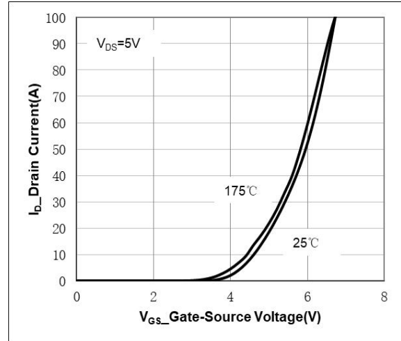
Fig 2 Transfer Characteristics
