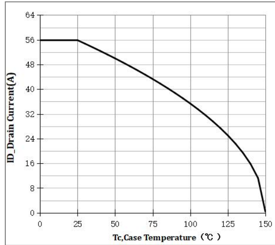
Fig 6 Current De-rating
