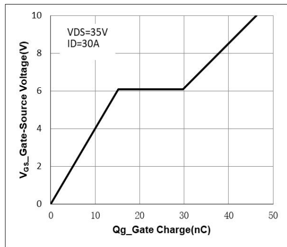
Fig 8 Gate Charge
