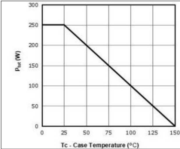
Figure 7 Power De-rating
