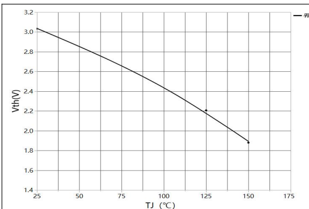
Figure 11 gate threshold voltage
