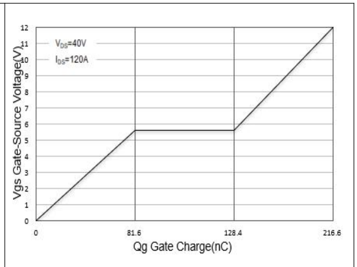
Figure 4 Gate Charge
