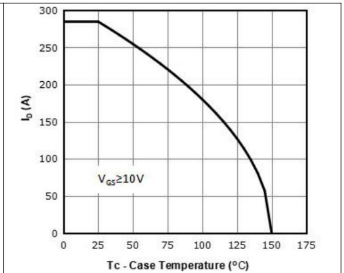
Figure 10 Current De-rating
