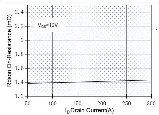
Figure 5 Rdson-Drain Current
