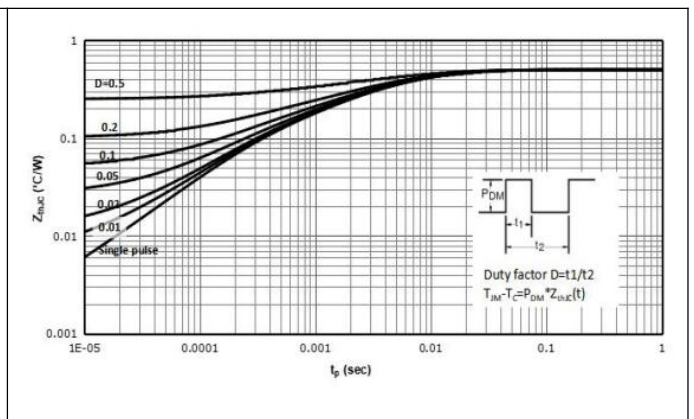
Figure 12 Normalized Maximum Transient Thermal Impedance
