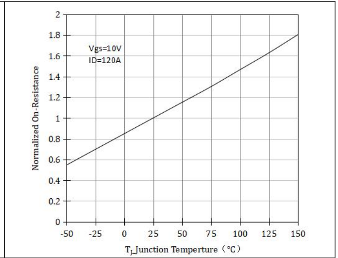
Figure 2 Rdson-Junction Temperature
