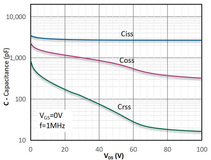
Fig6. Capacitance Characteristics
